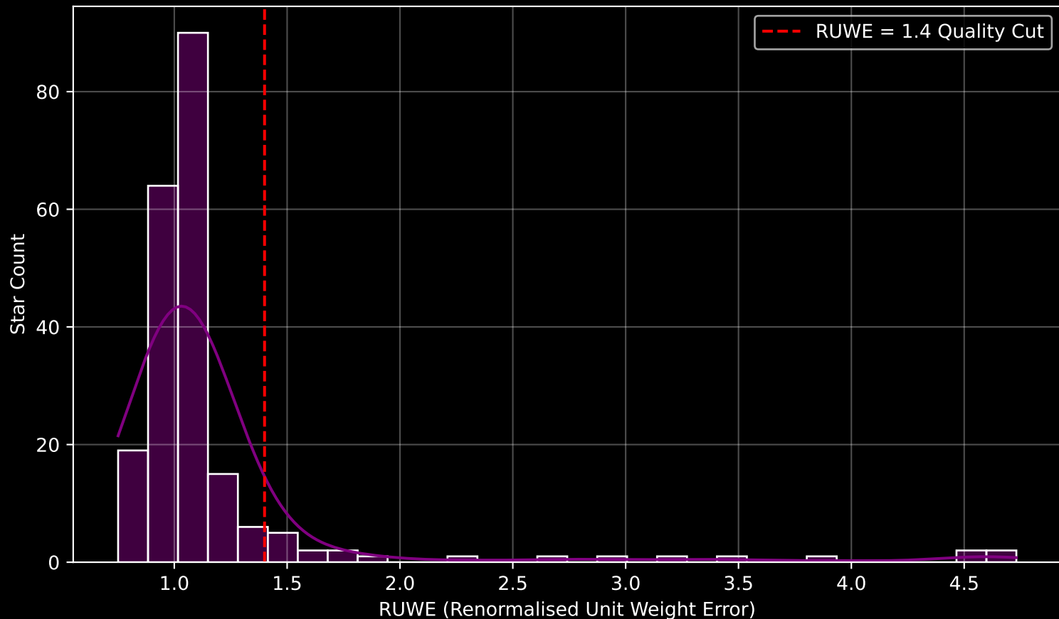
GAPOGEE DR17 Field [K2_C12_076-66_btx] RUWE Distribution (n= 214)
