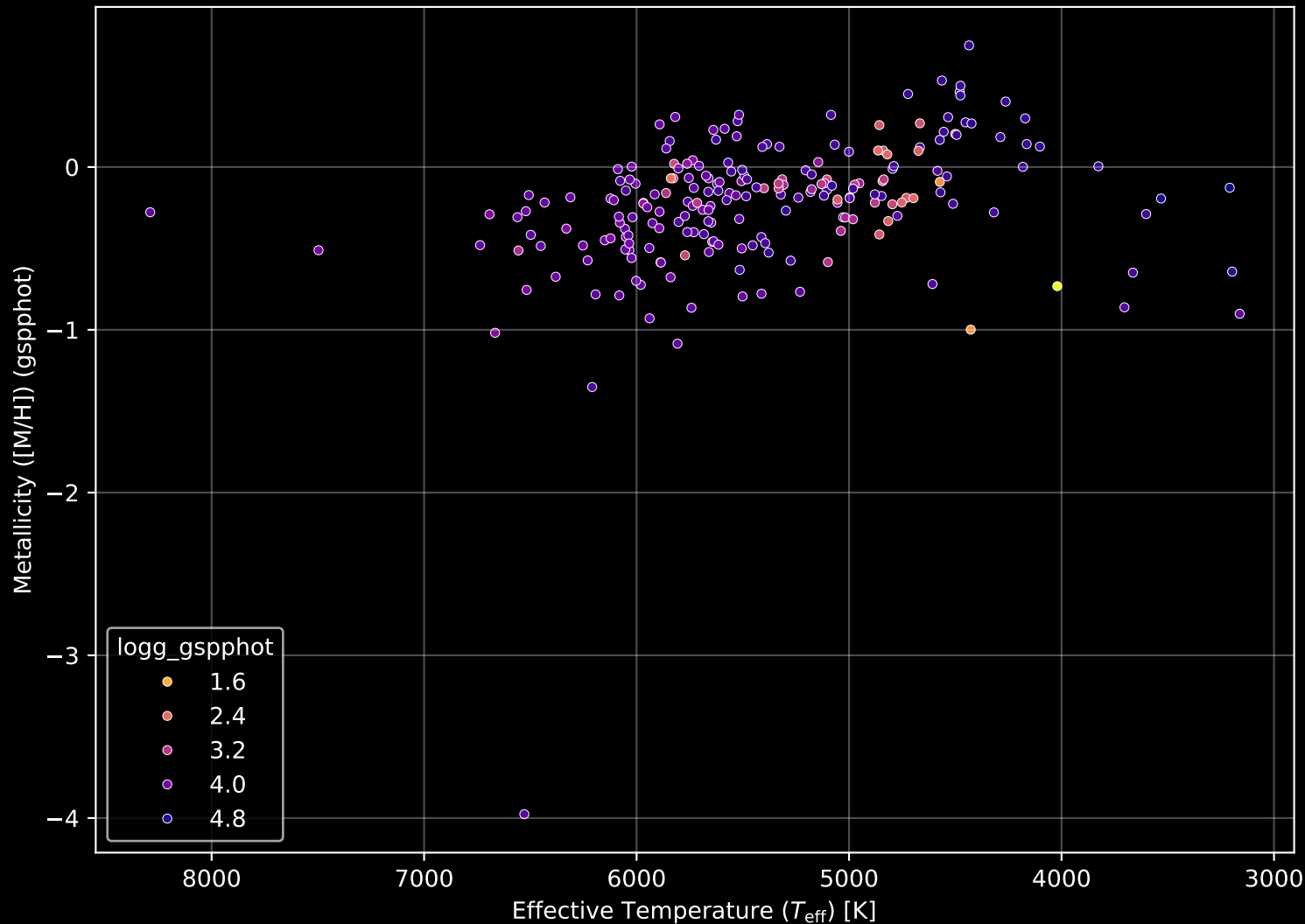
APOGEE DR17 Field: [K2_C12_076-66_btx] Stellar Population Parameters (n= 219)
