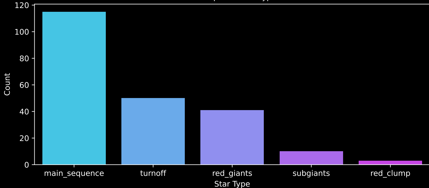
APOGEE DR17 Field: [K2_C12_076-66_btx] Count plot of Star Type
