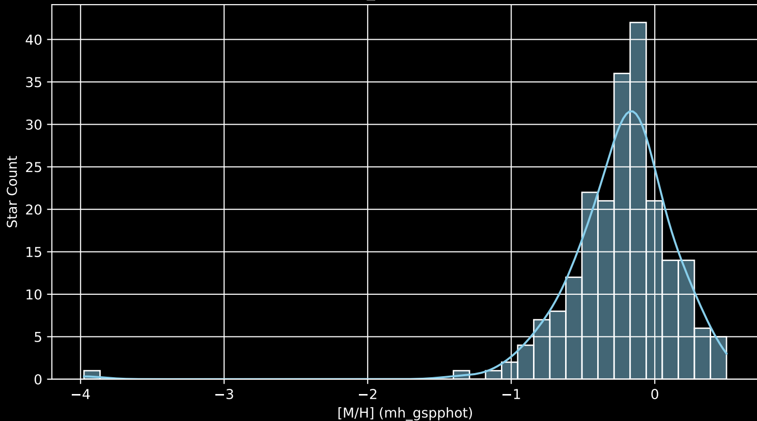
APOGEE DR17 Field: [K2_C12_076-66_btx [M/H] (mh_gspphot) (n= 217)
