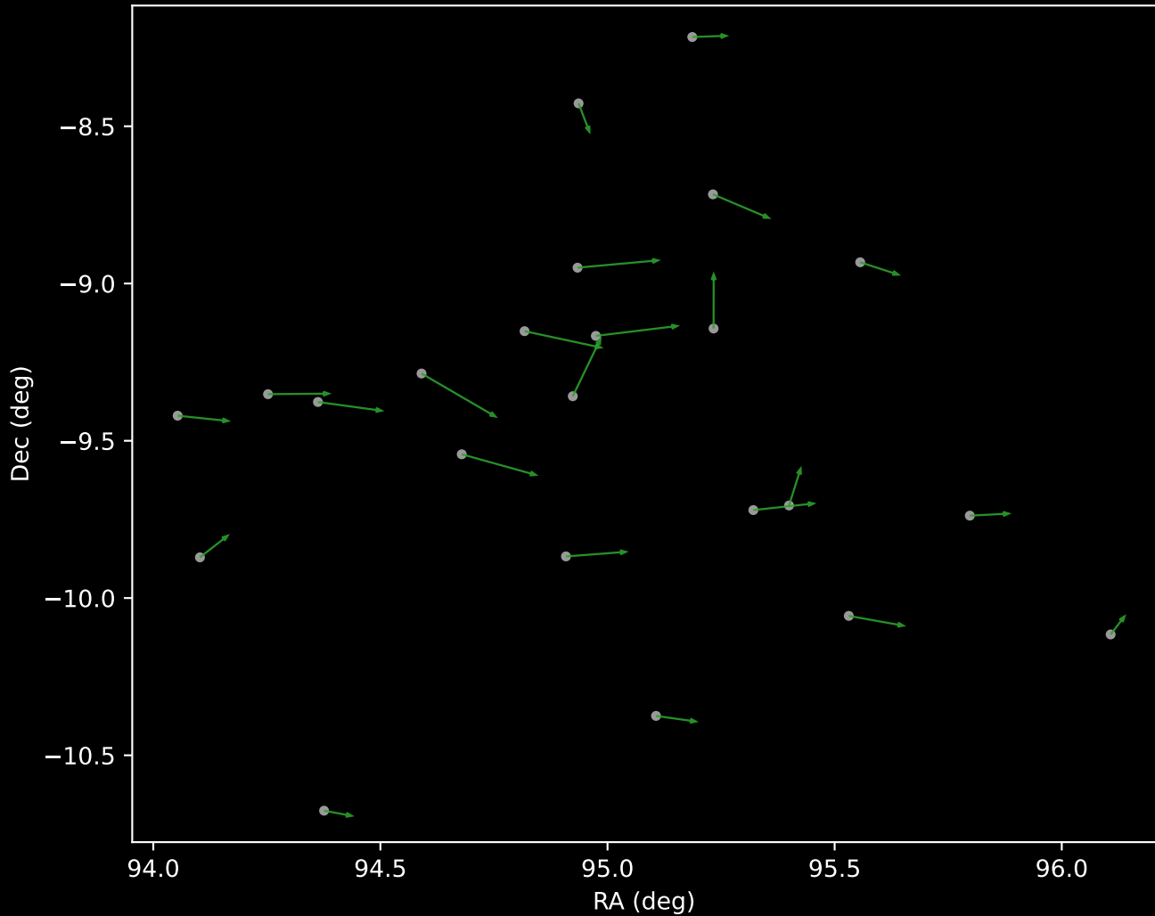
APOGEE DR17 Cluster 4 Proper Motion Vectors (n=23)
