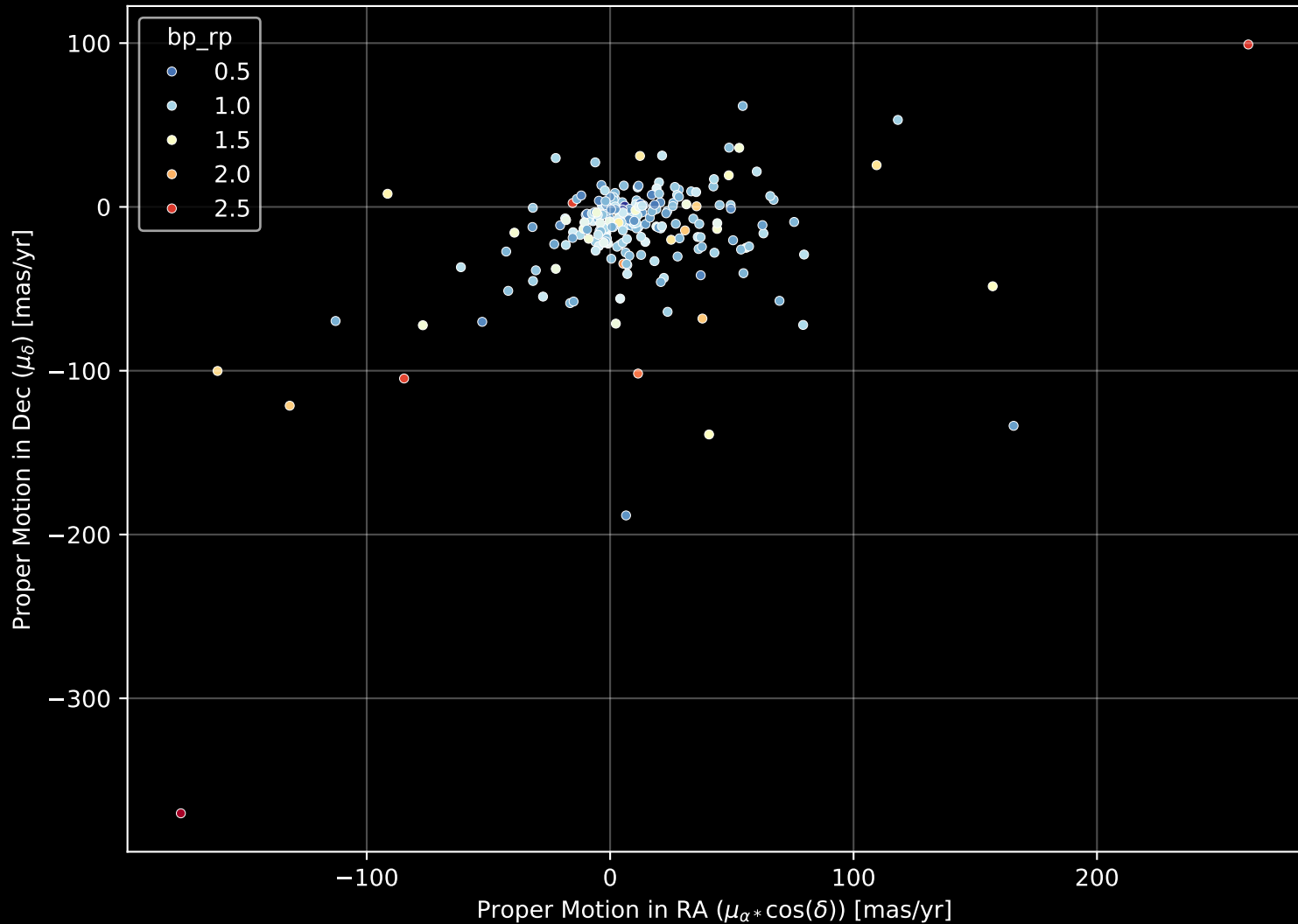
APOGEE DR17 Field: [K2_C12_076-66_btx] Proper Motion Diagram (n= 219)
