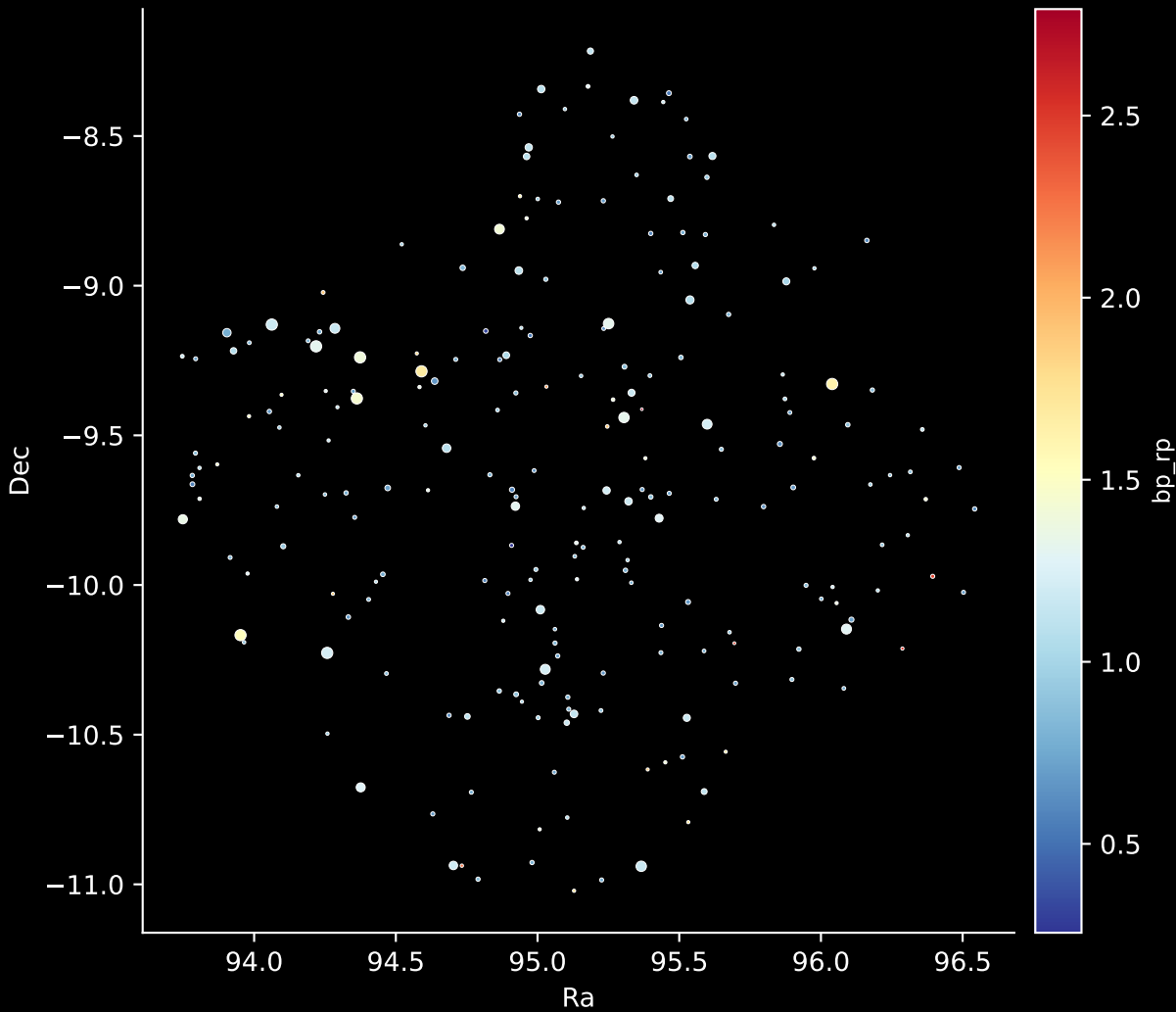
APOGEE DR17 Field: [K2_C12_076-66_btx] Stars: 219
