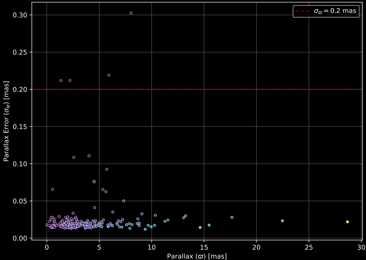
APOGEE DR17 Field: [K2_C12_076-66_btx] Parallax Quality (n= 219)
