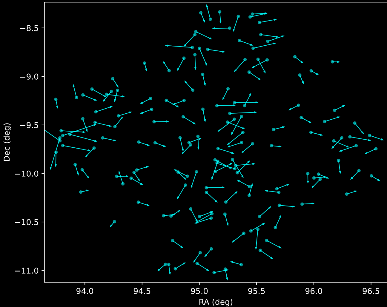
APOGEE DR17 Noise Stream Proper Motion Vectors (n=154)
